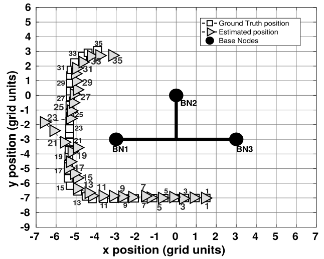
Fig. 15. Experimental results from one of the trials of the alternative averaging with variable-R approach. The plot shows the MN’s estimated position plotted against the ground truth.
